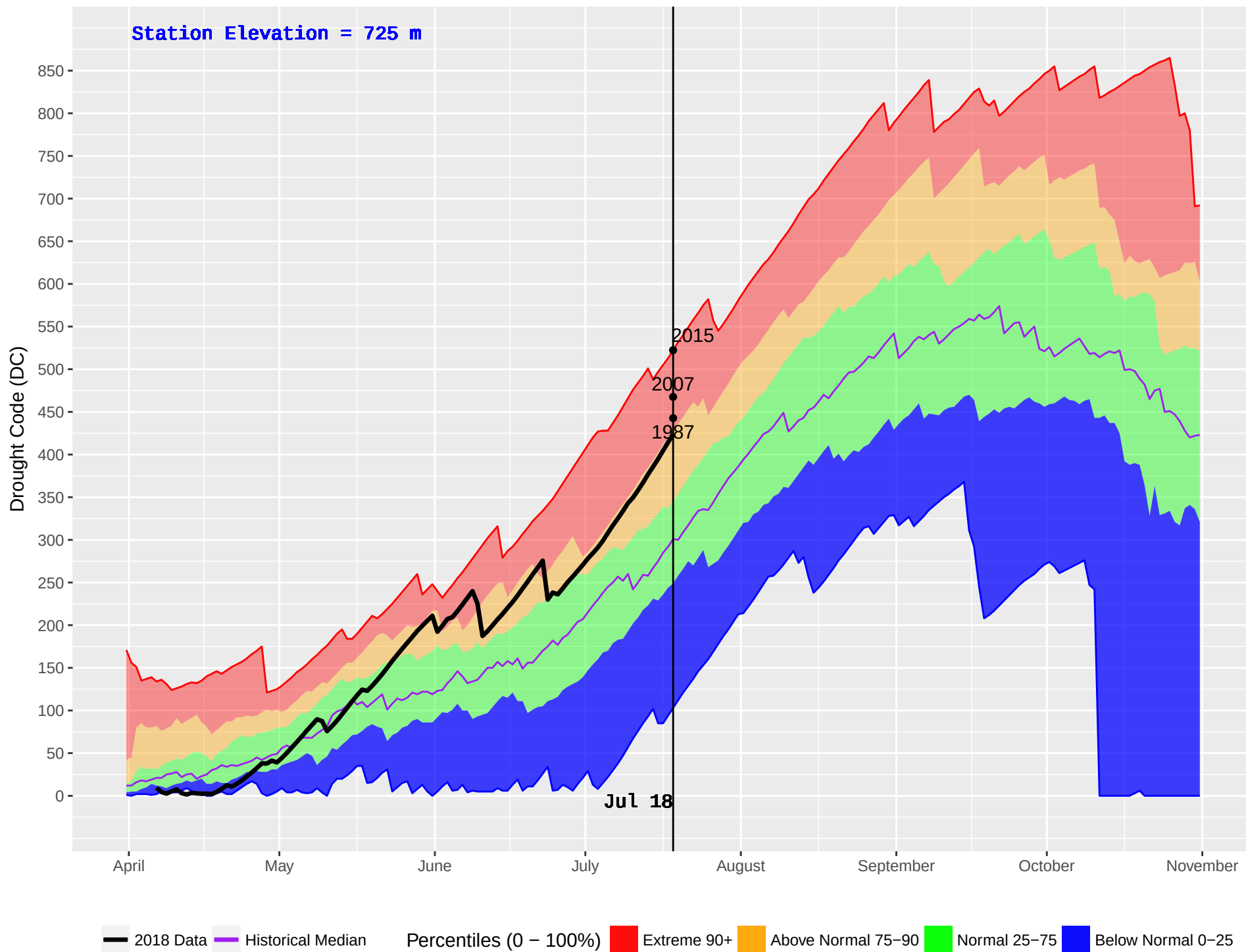
PENDOREILLE (402) : Historical (1986–2016) and Current (2018) Daily Drought Code (DC)
